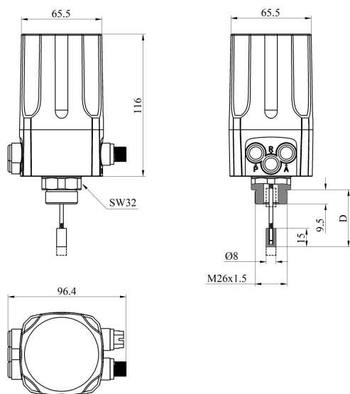
Sensor dimension for separate type
