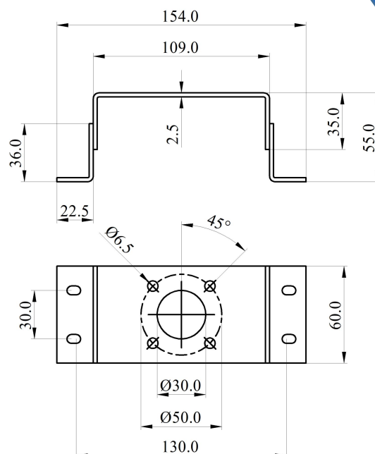
Rotary mounting bracket (Type B)
