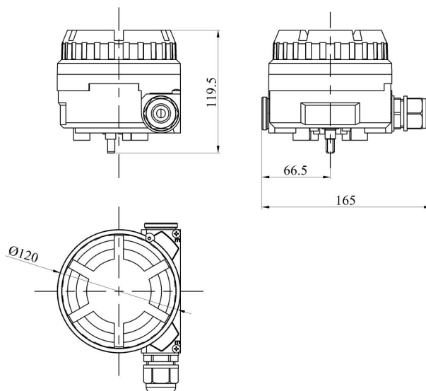
Sensor dimension for remote type
